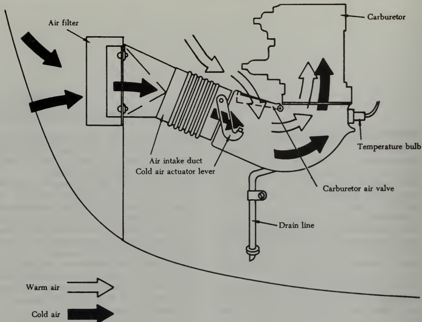
FIGURE 2-1. Nonsupercharged induction system using a carburetor.
